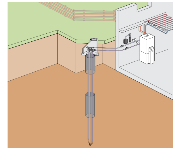
Vertical collector
