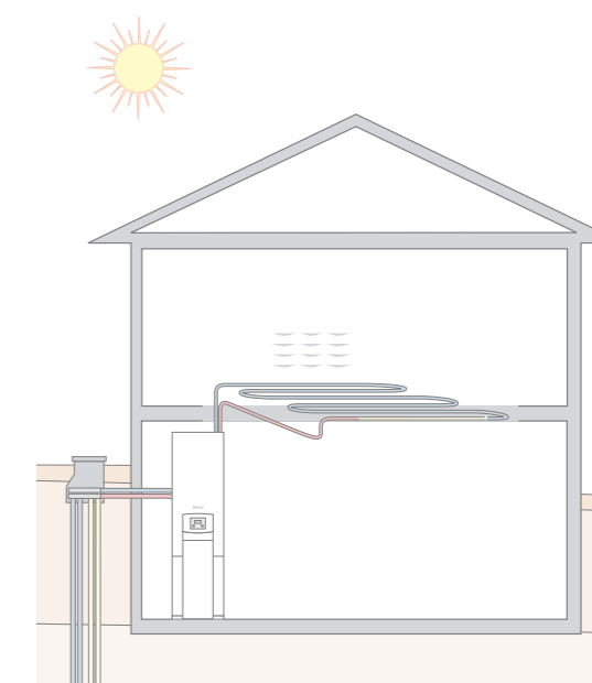
geoTHERM exclusive with passive underfloor cooling
