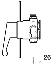
sola thermostatic shower valve - concealed
