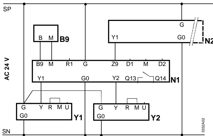
Extract air temperature control with heating and cooling, outside temperature compensation and minimum limitation of the supply air temperature
