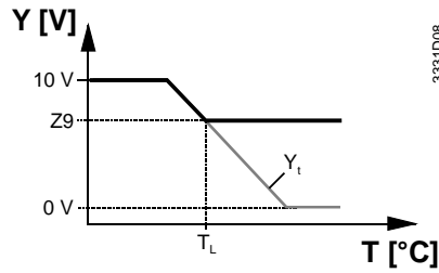
1-stage heating Minimum limitation of the controlled temperature
