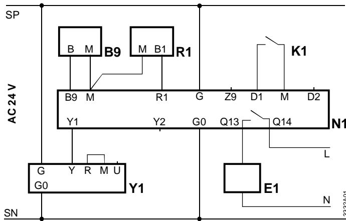
Supply air temperature control with outside temperature compensation, remote setpoint adjuster, setpoint changeover, and control of an auxiliary device
