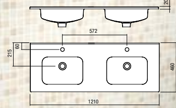
Basin MONZA 1210 porcelain white without drain pipe clicker
