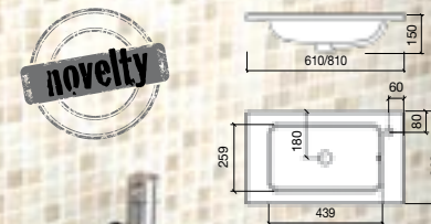
Basin NAPOLI 610 without drain pipe clicker
