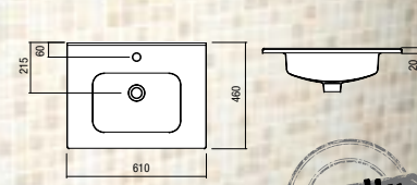
Basin MONZA 1210 porcelain white without drain pipe clicker
