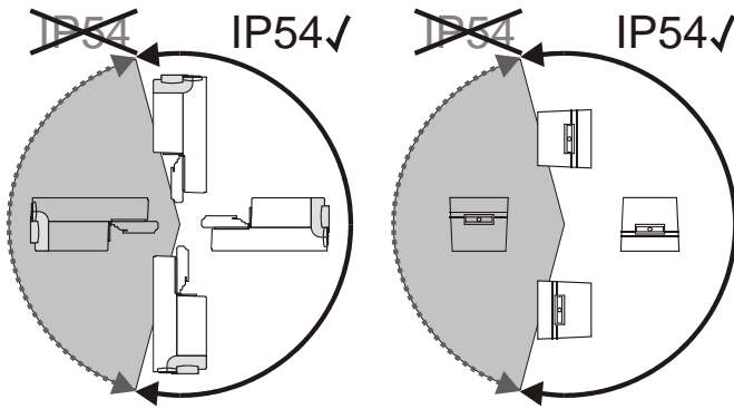
Fig. 9. Mounting for IP54
