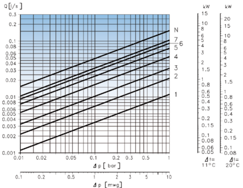
The pre-setting values 7 to 1 only apply for the pre-setting valve RA-N.
