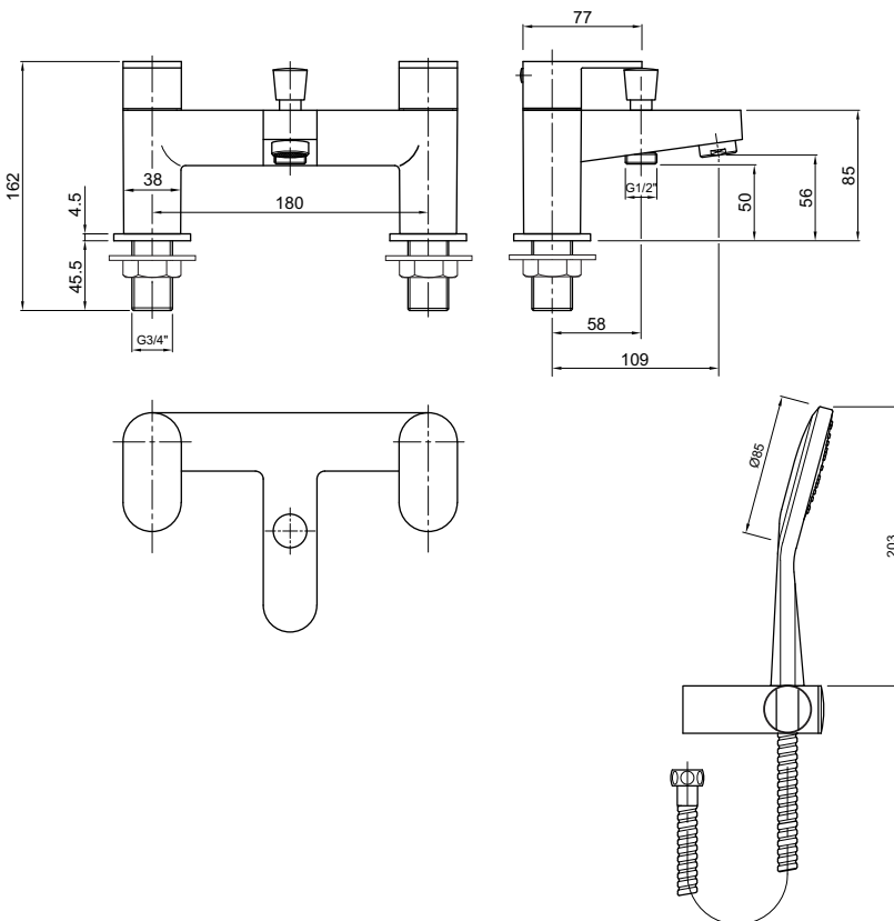
X70 Bath Shower Mixer Deck Mounted
