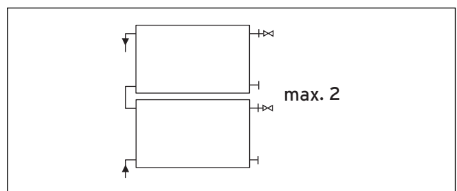
Fig. 4.5 Field arrangement on top of each other
