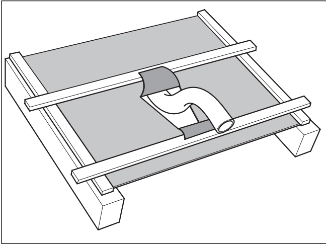
Fig. 4.7 Passing the pipe through the sarking membrane
