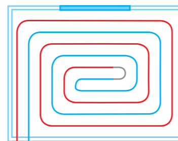
Counterflow
