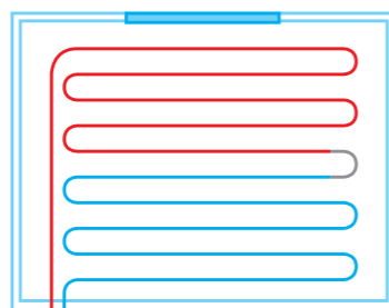
Single Serpentine
