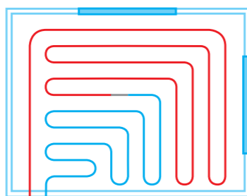
Double Serpentine
