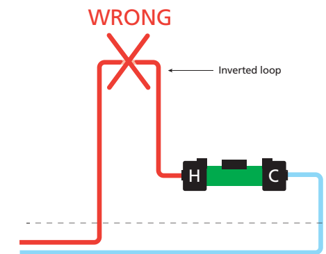
Figure 31: Inverted loops
