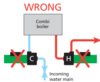
Figure 27: Combi boilers
