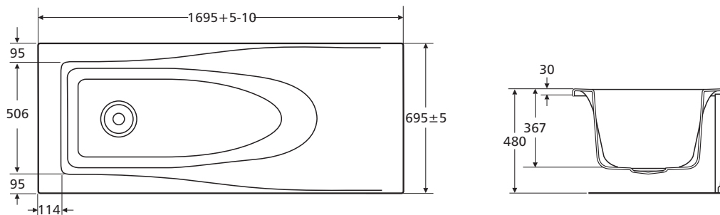
First 1700 x 700 rectangular bath
