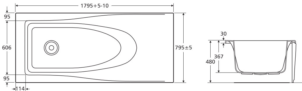
First 1800 x 800 rectangular bath
