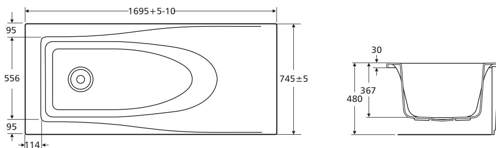
First 1700 x 750 rectangular bath
