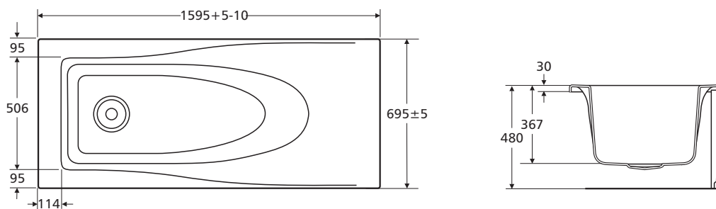
First 1600 x 700 rectangular bath
