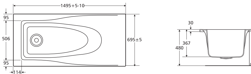
First 1500 x 700 rectangular bath
