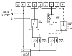
425 Tiara controlling fully pumped system using room stat, cylinder stat and two (2 port) spring return zone valve with auxiliary switches.
