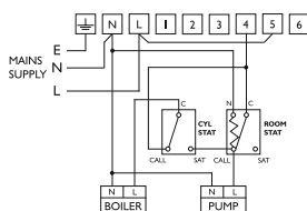
425 Coronet controlling gravity hot water with pumped heating via room stat and cylinder stat.
