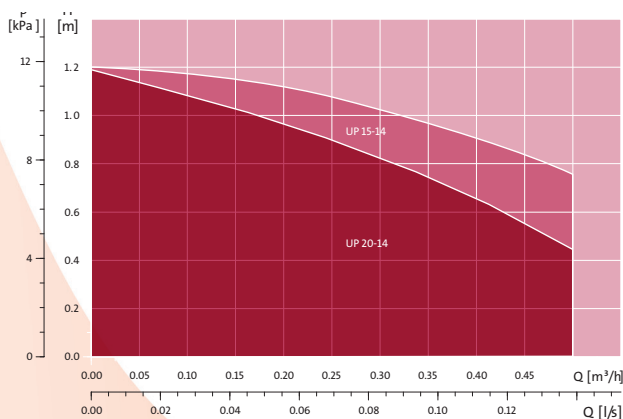
Performance curves for the COMFORT range.
