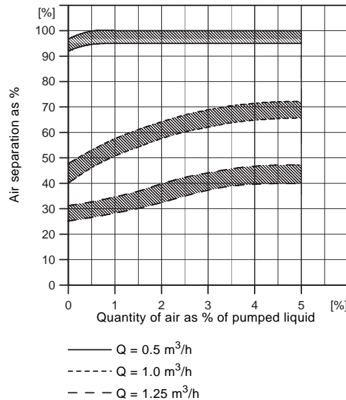
Fig. 14 Air separation
