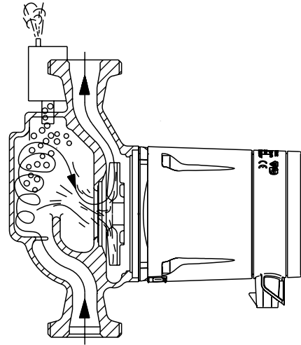
Fig. 13 Pump housing with air-separating chamber
