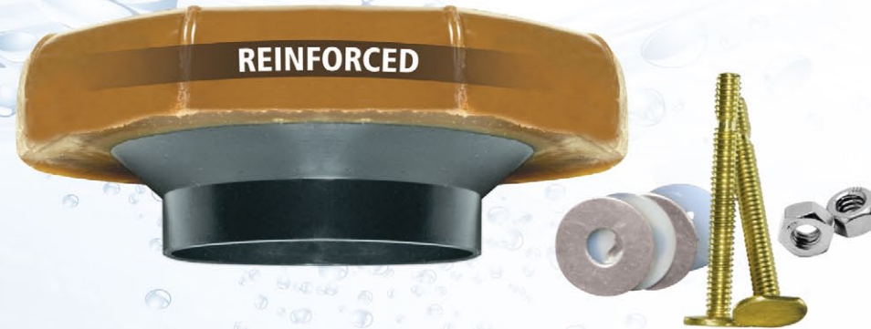
Reinforced Gasket with Flange 7512 Provides better seal on uneven flooring.
