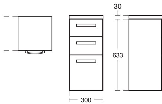
E2795 300 x 300mm base storage unit with three drawers
