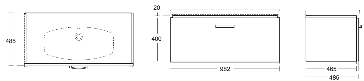
E2788 1000mm Countertop washbasin unit
