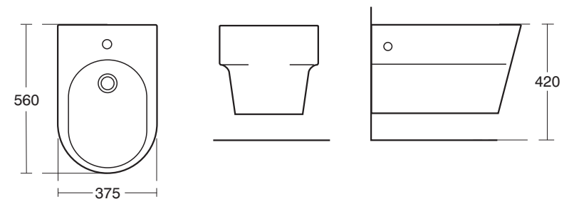
J4417 01 Wall Mounted Bidet
