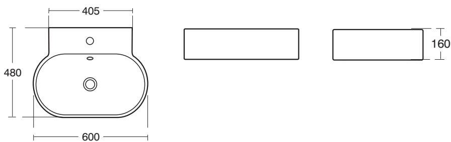
J4410 01 60cm Basin
