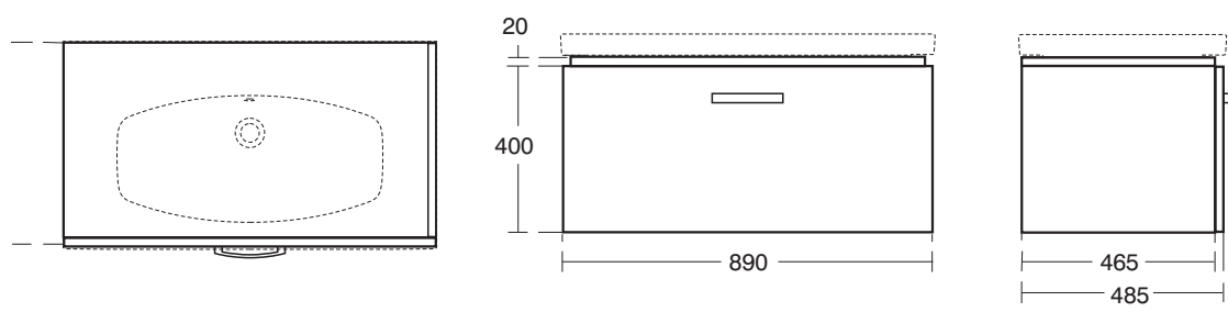
E2787 900mm Countertop washbasin unit
