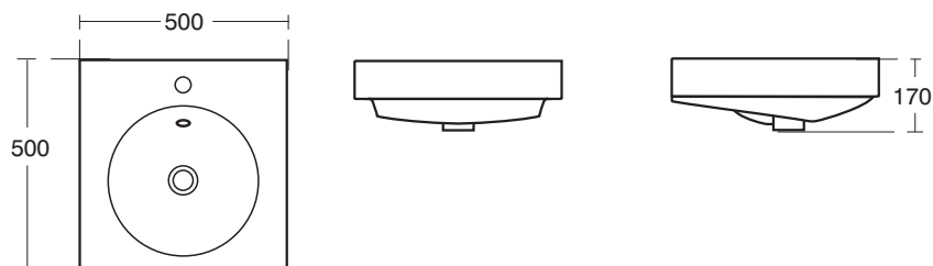
J4404 01 50cm Square Basin J4406 AA Lagaro Towel Rail for 50cm square basin J4408 AA Lagaro Towel Rail & Shelf for 50cm square basin
