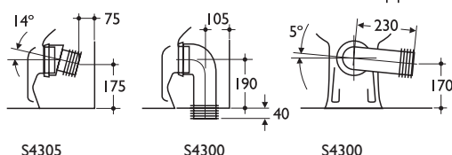
Conversion bends outlet to suit 102 bore soil pipe
