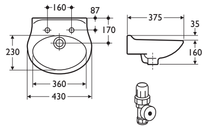
S2736 Sandringham Classic 43cm Handrinse Washbasin
