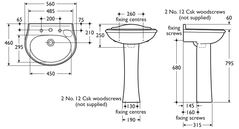
S2033 Sandringham Classic 56cm Washbasin
