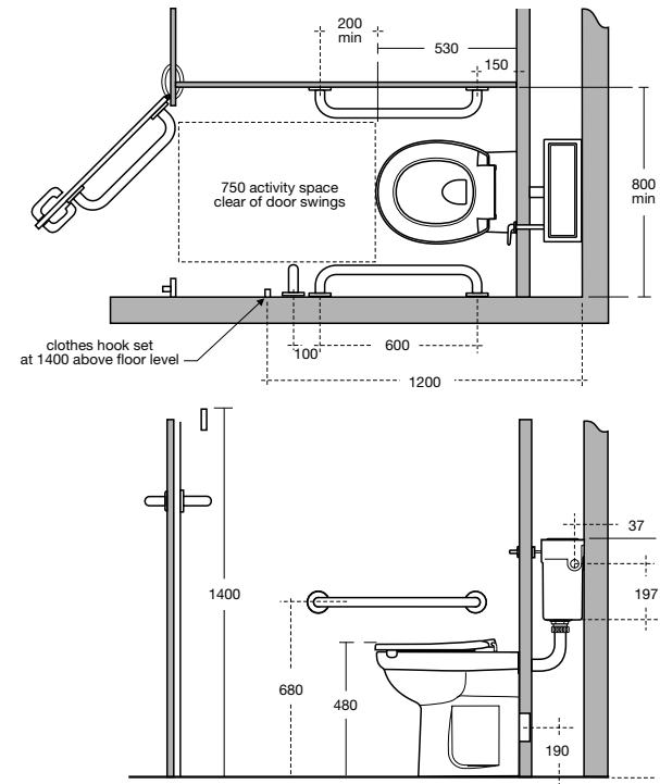
Back-to-wall WC suite detail (above).
