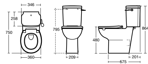
Close coupled WC suite detail (above).
